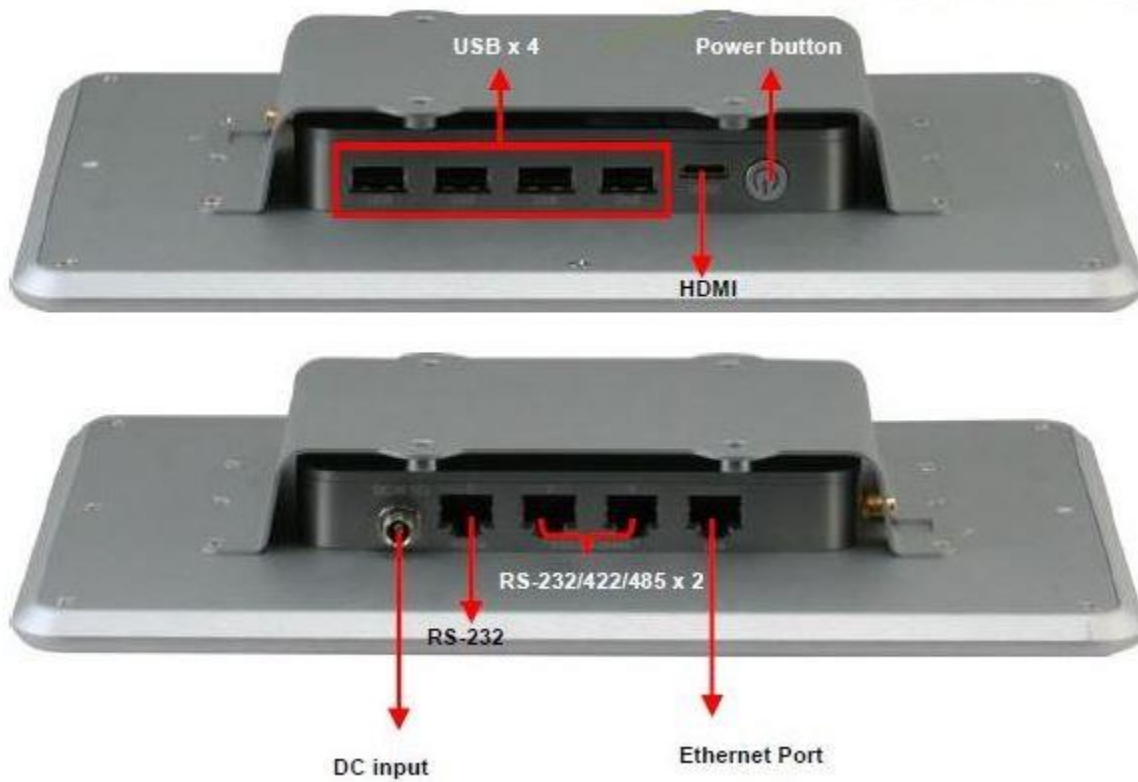
Figure 1. c-WashPal Connection Locations
